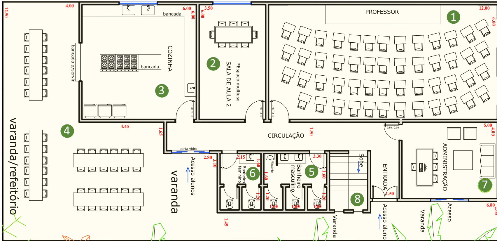
Ground Floor
